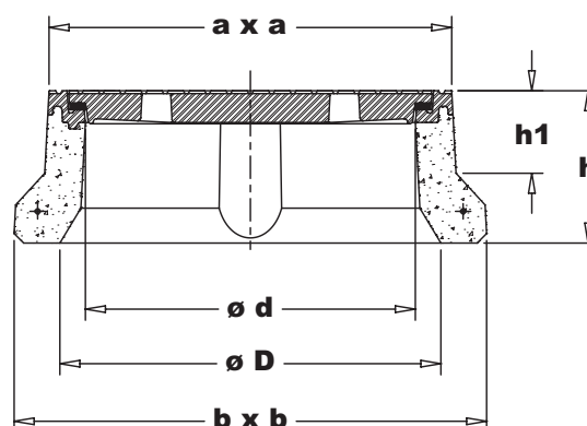
type N 362 NB-RR Centernorm
